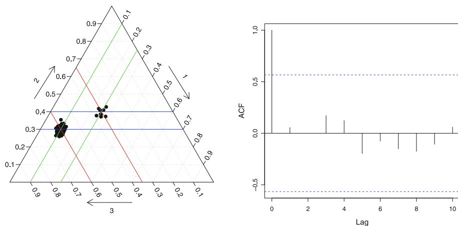
Fig. 3 Left : example of the vectors X_i in the simplex at time t_1 for the random dot process model, with n = 100 , n_1 = 9 , K = 2 , \pi_0 = (0.10, 0.30, 0.60)^T and \pi_1 = (0.25, 0.40, 0.35)^T . (The matrices Q_0 and Q_1 are given in Sect. 4.2.2.) For this case (with r = 1024 —see Sect. 3.1) the second approximation (truncated multivariate normals) provides a good model. Right : autocorrelation as a function of lag for the edge attributes, showing that (for this case) the graphs are approximately uncorrelated in time
