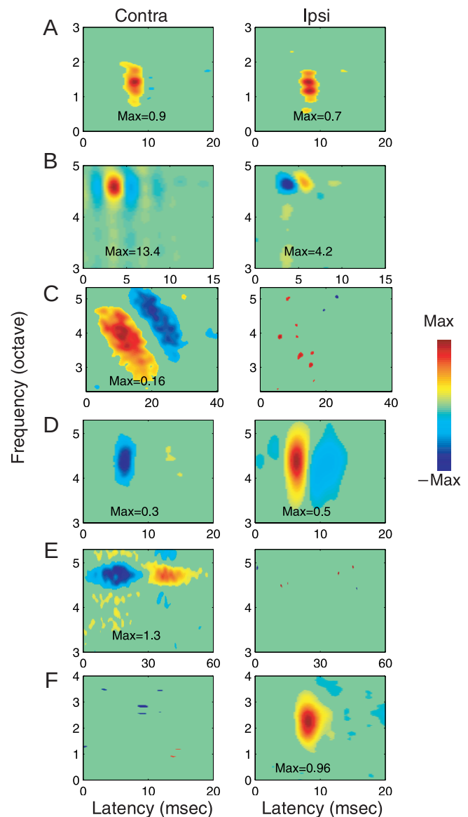
FIG. 13. Representative binaural STRFs. Contralateral ( left ) and ipsilateral ( right ) STRFs exhibited a variety of arrangements of spectral and/or temporal excitation and/or inhibition, although all binaural receptive fields showed a large degree of spectro-temporal overlap. Only STRF subregions that exceeded significance ( P < 0.002 ) are shown. Neurons could exhibit purely excitatory interactions ( A ), excitatory and inhibitory interactions ( D and B ), or could respond exclusively to the contra- or ipsi-ear ( C , E , and F ).
