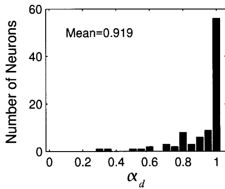
FIG. 12. Distribution of separability index ( \alpha_d ). Most neurons (56/93) have perfectly separable time-frequency structure ( \alpha_d = 1 ). The mean separability index (0.919) is exceptionally high, indicating that most collicular STRFs are well approximated by the product of the TRF and SRF profile.
