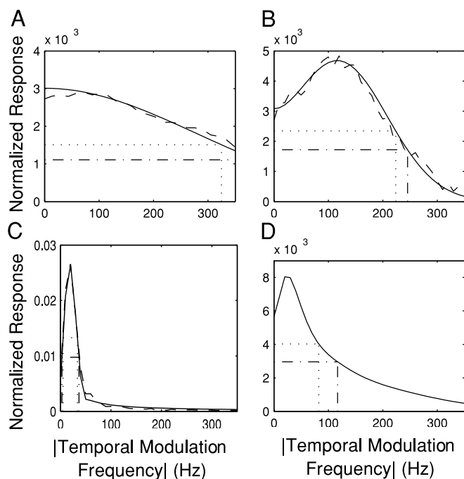
FIG. 10. Representative temporal modulation transfer functions (tMTFs). — and ---, the fitted and measured tMTFs (normalized for unit energy), respectively. A and B: typical lowpass tMTFs with 0 (A) and non-0 (B) best temporal modulation frequencies (bandwidths, A: 350 Hz at upper 8.68 dB cutoff; 324.7 Hz at 6 dB upper cutoff; B: 245.4 Hz at upper 8.68 dB cutoff; 223.8 Hz at upper 6 dB cutoff). C: a typical bandpass tMTF (best temporal modulation frequency: 20.0 Hz; bandwidth: 34.0 Hz at upper 8.68 dB cutoff; 28.5 Hz at upper 6 dB cutoff). D: the composite population tMTF for the ICC is lowpass in character with non-0 best temporal modulation rate (30.0 Hz; bandwidth: 117.0 Hz at upper 8.68 dB cutoff; 82.5 Hz at upper 6 dB cutoff). ··· and - · - ·, the upper 6 dB and 8.68 dB cutoff, respectively.
