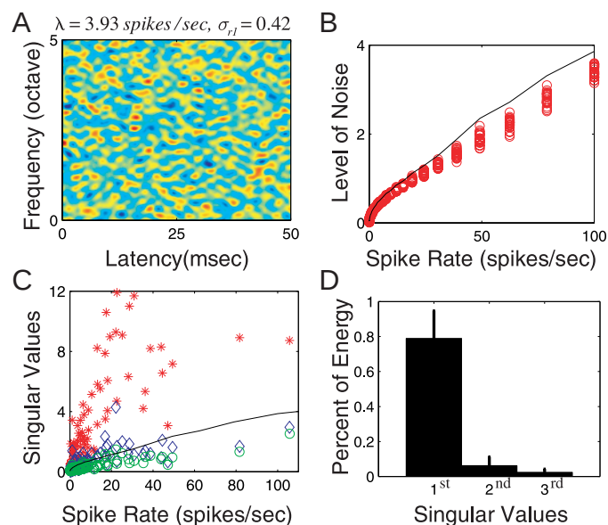
FIG. 4. Significance analysis of the Gabor STRF model. A random noise STRF, STRF_r (A), is generated by reverse-correlating the dynamic moving ripple sound and a random, Poisson-distributed spike train at a specific spike rate ( \lambda = 3.93 spikes/s for this example). The noise level is obtained by measuring the first singular value ( \sigma_{r1} = 0.42 for the shown example) of the STRF_r with the SVD method used to break up the STRF into separable components (Fig. 3). For each spike rate this procedure is resimulated 25 times to estimate the distribution of noise-levels (vertical red circles in B). A resampling bootstrap technique is used to estimate the threshold-level required to achieve a significance of P < 0.01 at each spike rate (continuous line, B and C). The relationship between the noise-threshold level, the measured spike rate and the 1st, 2nd, and 3rd singular values obtained from the STRFs of all neurons is depicted in (C). All of the 1st-singular values (100%) exceed the noise threshold (red *), whereas only 39.7% of the 2nd (blue \diamond ), and 7.5% of the 3rd singular (green \circ ) values exceed significance ( P < 0.01 ). Energy contribution of the separable STRF component (D). The 1st STRF component, ( STRF_1 ) accounts for 78.9 \pm 15.7\% (mean \pm SD) of the STRFs energy. The contributions of the 2nd ( 6.2 \pm 5.0\% ) and 3rd ( 2.3 \pm 1.8\% ) STRF components is significantly smaller.
