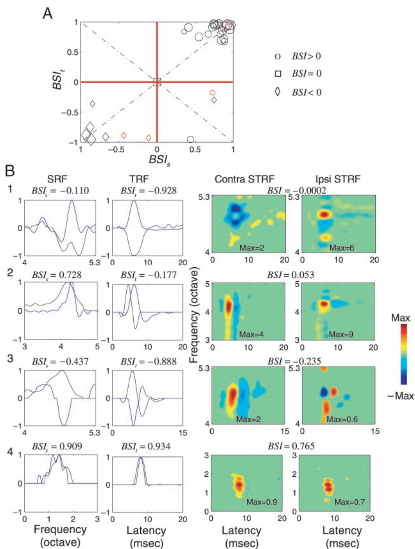
FIG. 14. Analysis of binaural receptive field disparity. A : the joint distribution of spectral (BSI s ), temporal (BSI t ), and spectro-temporal (BSI) binaural similarity indexes. Spectral and temporal BSIs are designated along the abscissa and ordinate, respectively, whereas the magnitude and sign of the spectro-temporal BSI are represented symbolically by symbols of different sizes (open diamonds and open circles indicate BSI < 0 and BSI > 0, respectively; larger symbols corresponds to larger BSI magnitudes). Neurons with 0 BSI showed only monaural preferences (open squares symbol). B : example neurons showing various spectral, temporal, and spectro-temporal receptive field arrangements (denoted by red symbols in A ). Neurons can exhibit correlated (e.g., neuron 4), uncorrelated (e.g., neuron 1, 2), or anticorrelated (e.g., neuron 1–3) spectral and/or temporal receptive field structures. Receptive field data is shown at a significance level of P < 0.002 .
