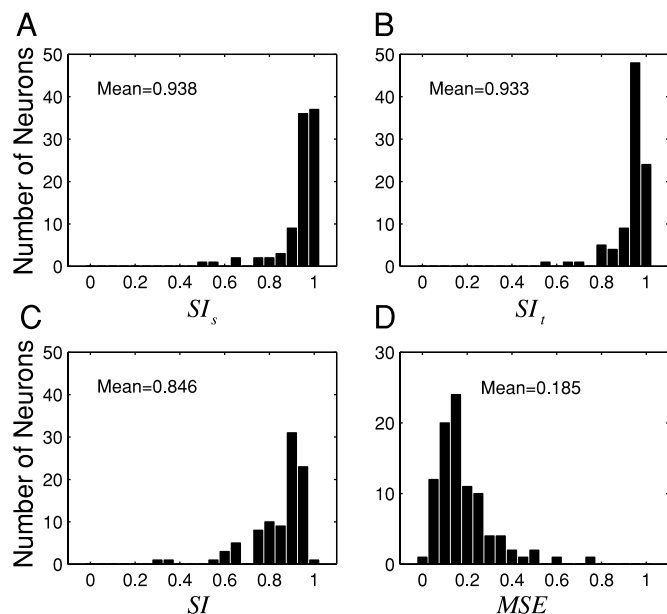
FIG. 6. Gabor STRF error analysis. Distribution of spectral similarity index ( SI_s ; A), temporal similarity index ( SI_t ; B), STRF similarity index ( SI ; C), and the energy error metric (MSE; D). The spectral and temporal SI quantify shape similarity between the measured and modeled SRF and TRF profiles, respectively. Both means are near unity suggesting that the Gabor model can adequately account for the shape of the SRF and TRF profiles. The STRF similarity index, assumes values that are slightly lower than for the SRF and TRF (C) because shape errors from the Gabor TRF and SRF models are propagated to the Gabor STRF model. The overall goodness of fit was measured with the energy error metric (lower values correspond to better fits), which typically assumed small values (D).
