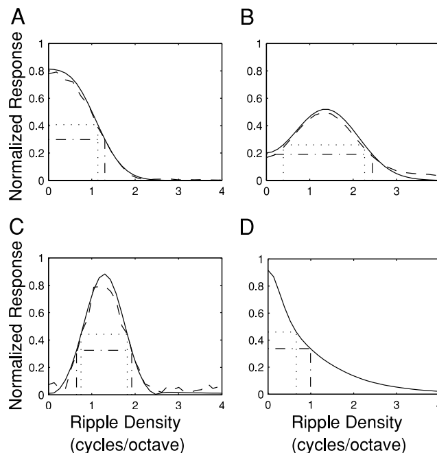
FIG. 8. Representative spectral modulation transfer functions (sMTF). — and ---, the fitted and measured sMTFs, respectively. All sMTFs are normalized for unit energy. A: a typical lowpass sMTF with the best ripple density ( \Omega_0 = 0 cycles/octave) and bandwidth (1.30 cycles/octave at upper 8.68-dB cutoff or 1.14 cycles/octave at upper 6-dB cutoff). B (best ripple density: 1.30 cycles/octave; bandwidth: 2.44 cycles/octave at upper 8.68-dB cutoff; 1.87 cycles/octave at upper 6-dB cutoff) and C (best ripple density: 1.30 cycles/octave; bandwidth: 1.27 cycles/octave at upper 8.68-dB cutoff; 1.07 cycles/octave at upper 6-dB cutoff) show typical sMTFs with bandpass filter characteristics. D: the composite population sMTF for the inferior colliculus (ICC) assumes a lowpass filter characteristic with a best ripple density of zero and bandwidth 0.995 cycles/octave (at upper 8.68-dB cutoff) or 0.662 cycles/octave (at upper 6-dB cutoff). ··· and - · - ·, the upper 6- and 8.68-dB cutoff, respectively.
