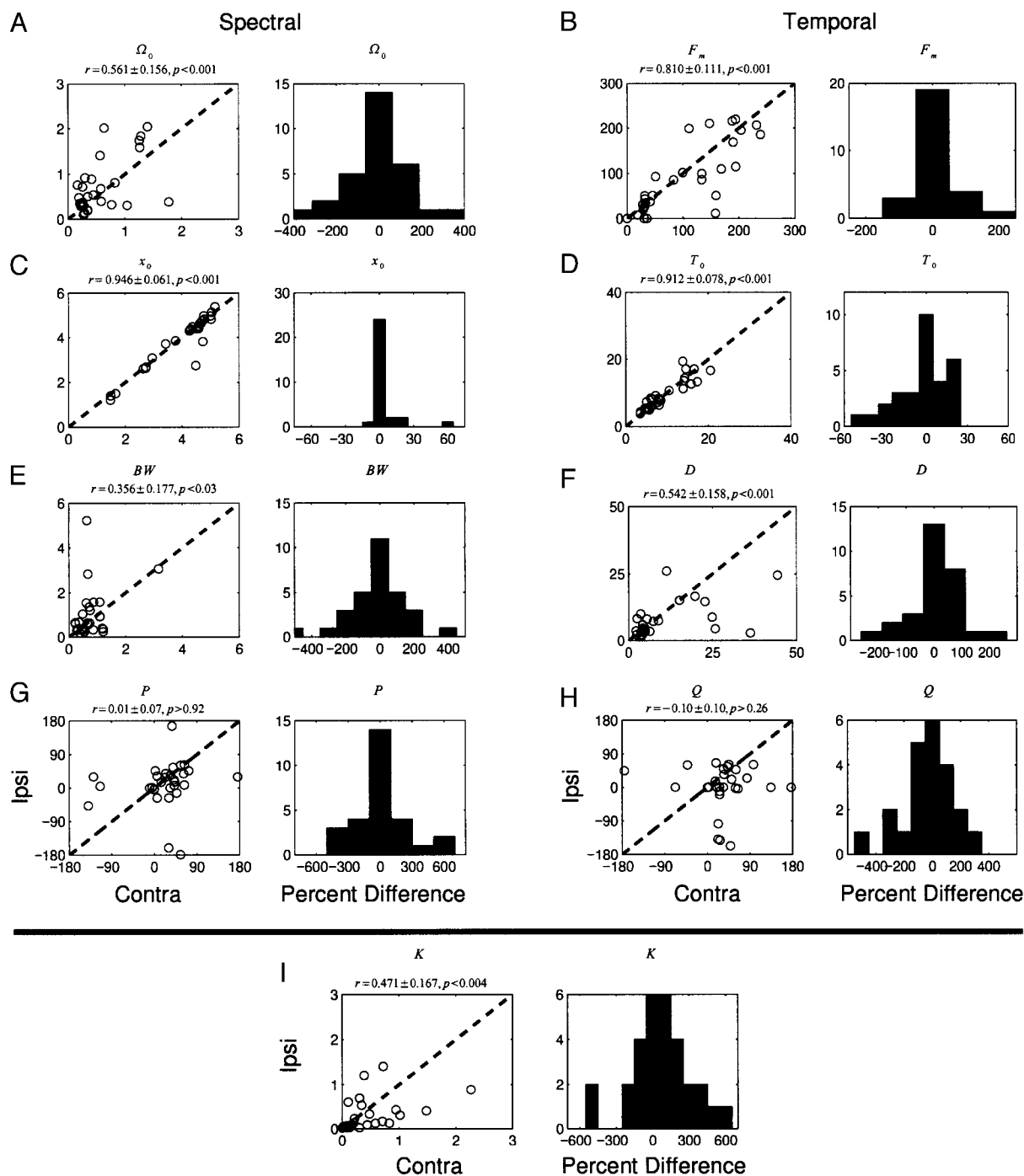
FIG. 15. Contralateral and ipsilateral receptive field parameter distributions. A–I: scatter plots and disparity distributions (percent difference between contra and ipsi) showing spectral (left) and temporal (right) parameters of the contra and ipsi receptive field: A: best ripple density ( \Omega_0 ); B: the best temporal modulation frequency ( F_m ); C: the center frequency ( x_0 ); D: the peak latency ( T_0 ); E: the bandwidth of the SRF profile (BW); F: the response duration (D); G: the spectral phase (P); H: the temporal phase (Q); and I: response strength (K), respectively. Correlation coefficients and the corresponding significance levels are indicated on top of each scatter plot.
