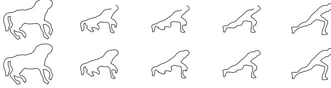
FIG. 7. Curve evolution with and without the closedness constraint. Lower and upper bounds for the geodesic distance: 0.498 and 0.532.
