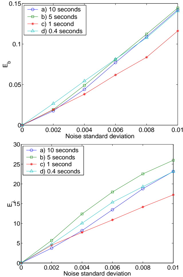
Fig. 2. Error in the estimation of the model parameters E_b and the discrete state E_\lambda for different levels of noise with standard deviation \sigma and for different dwell times: a) 10 seconds, b) 5 seconds, c) 1 second and d) 0.4 seconds.
