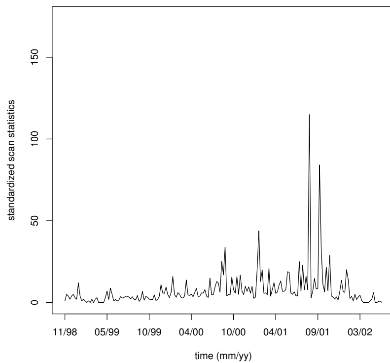
Figure 13: Time series of standardized scan statistic \widetilde{M}_{1,t} for weekly Enron email digraphs during a period of 189 weeks from 1998–2002. (See also Figure 2.)
