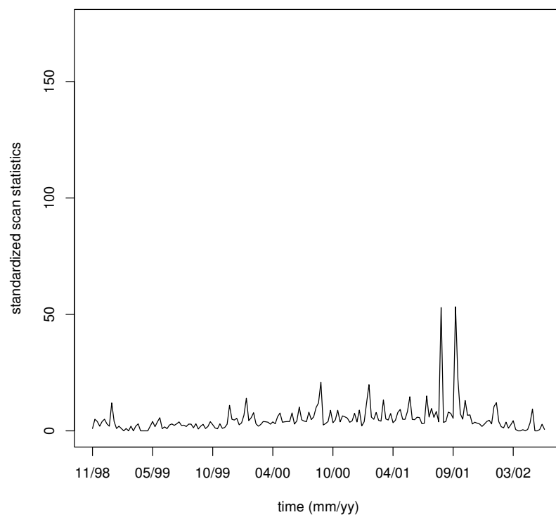
Figure 12: Time series of standardized scan statistic \widetilde{M}_{0,t} for weekly Enron email digraphs during a period of 189 weeks from 1998–2002. (See also Figure 2.)
