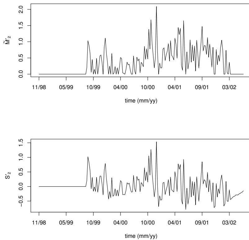
Figure 5: Plot of order 2 statistics \tilde{M}'_t and S'_t showing the maximum at t^* = 109 in December 2000. This is the email164 “excessive chatter” detection.
